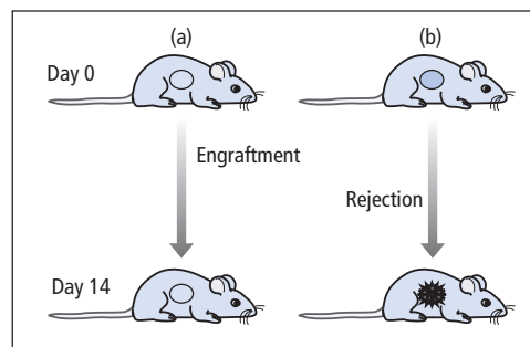
Figure 1.4 Discrimination between self and non-self illustrated by skin grafting in a rodent. (a) The graft was of 'self' type; (b) the graft was from an unrelated animal.
