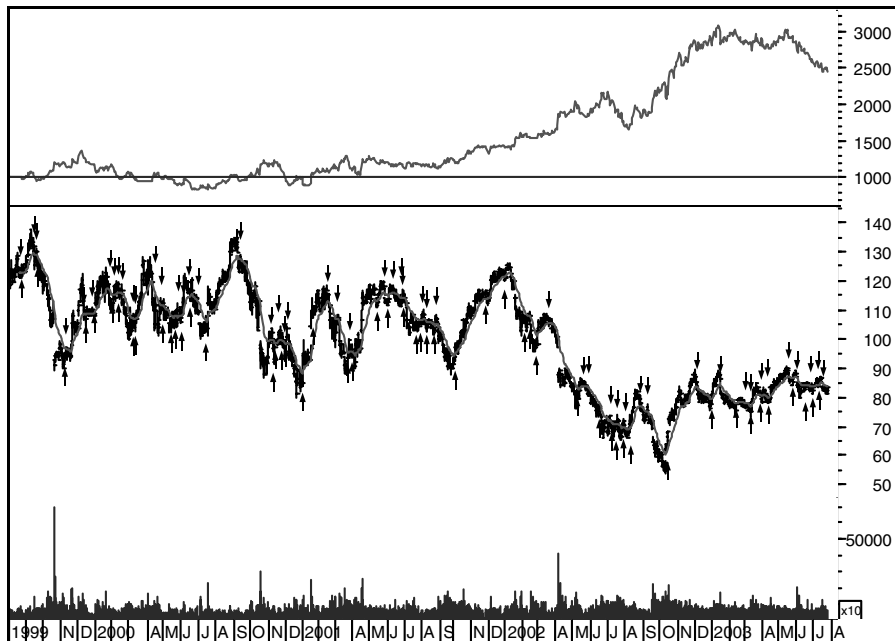
Figure 1-7: Optimization back-test.
