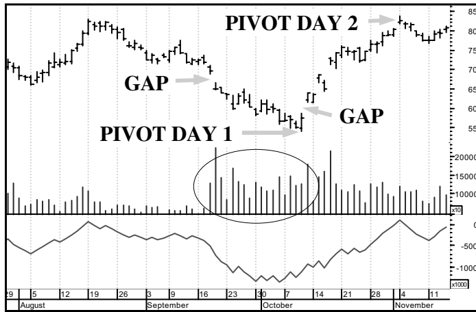
Figure 1-4: On-balance volume.
