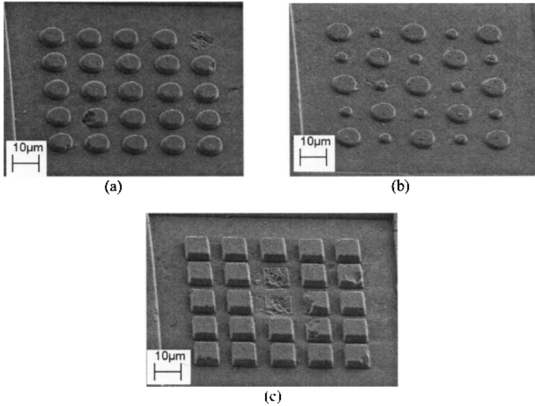
Figure 5. \text{Al}_2\text{O}_3 nanoparticle arrays produced from PDMS mold: (a) homogeneous round island array, (b) heterogeneous round island array, and (c) homogeneous square island array.
