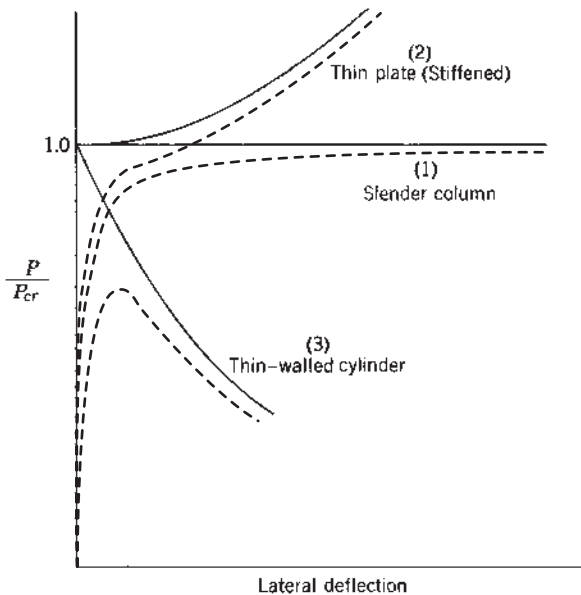
FIGURE 1.2 Elastic postbuckling curves for compressed elements.
