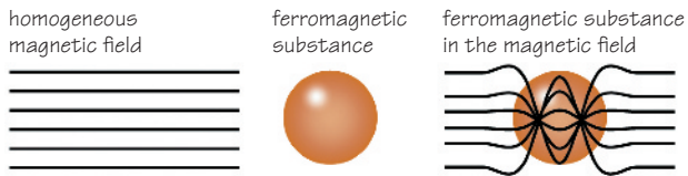
Figure 1.3 Ferromagnetic properties.
