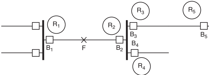
Figure 1.8 Reliability of protection system
