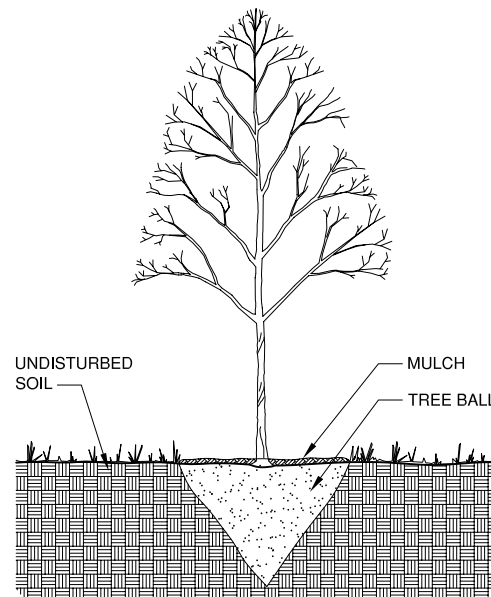
TYPICAL TREE SPADE BALL AND PLANTING PIT CONFIGURATION
