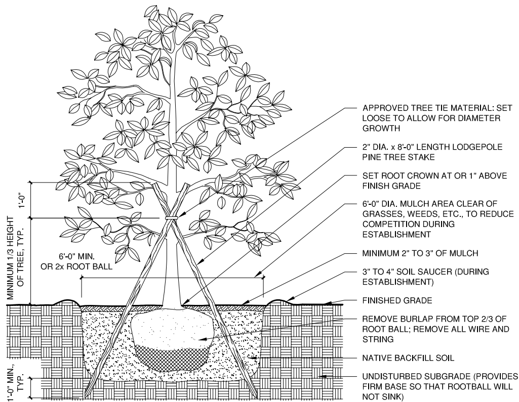
TWO ANGULAR STAKES
