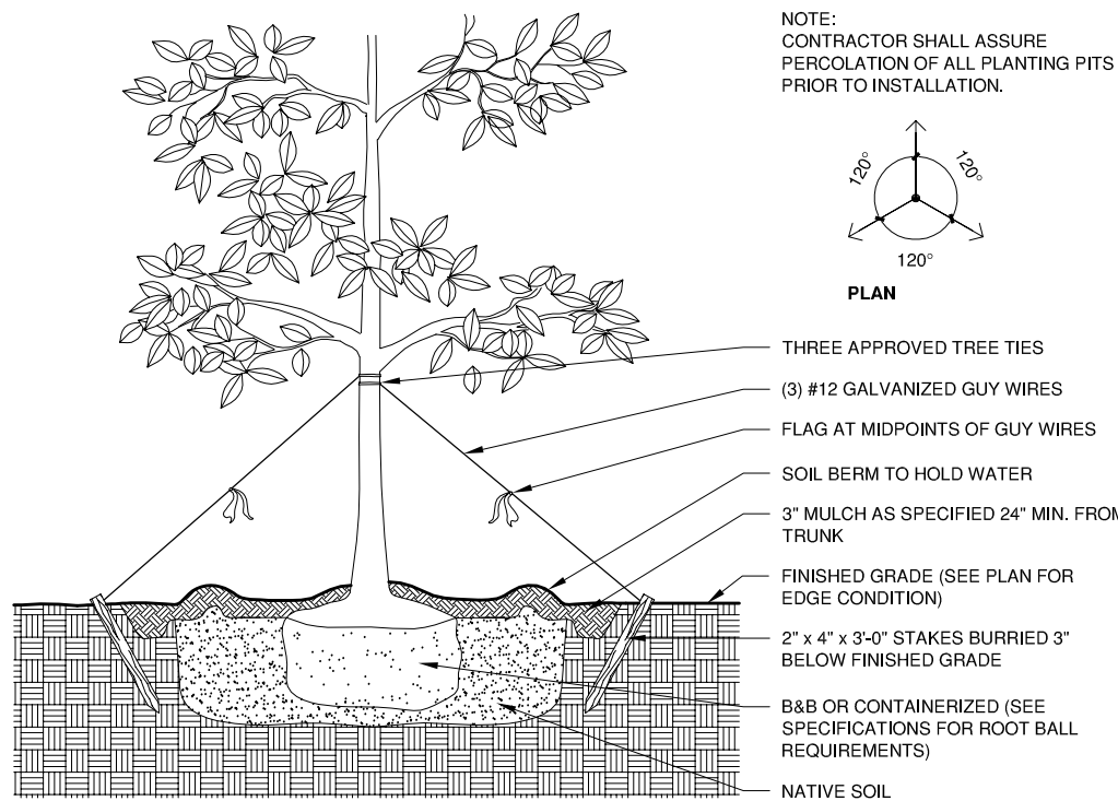
THREE GUY WIRE STAKING SYSTEM
